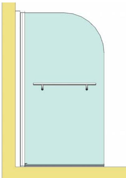
SS11 : CURVED SCREEN + TOWEL RAIL
